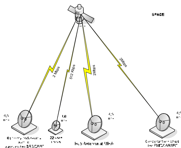
Figure 1: DMS Network
